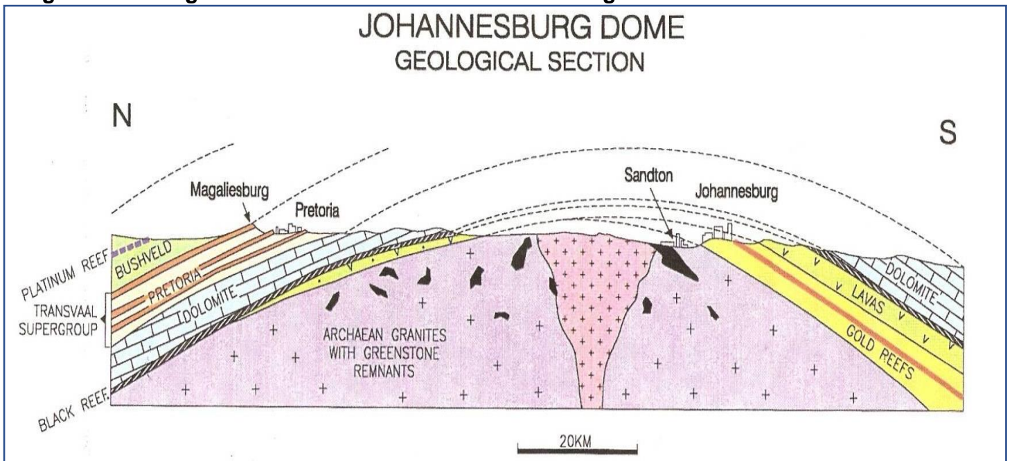
Figure 9: Geological Cross Section of the Johannesburg Dome
