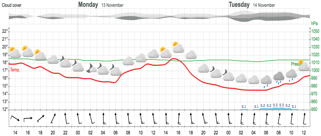
Figure 1: Meteogram of Cape Town
