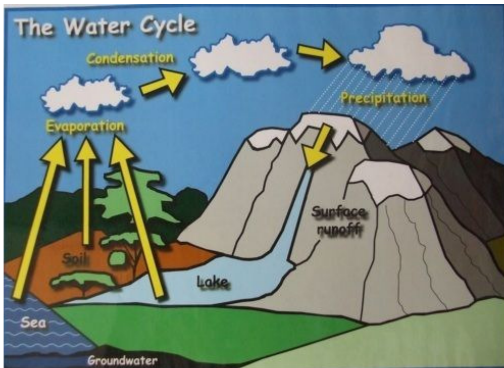
Figure 4: water cycle updated
